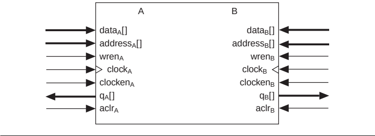
Figure 2–12. True Dual-Port Memory Configuration
