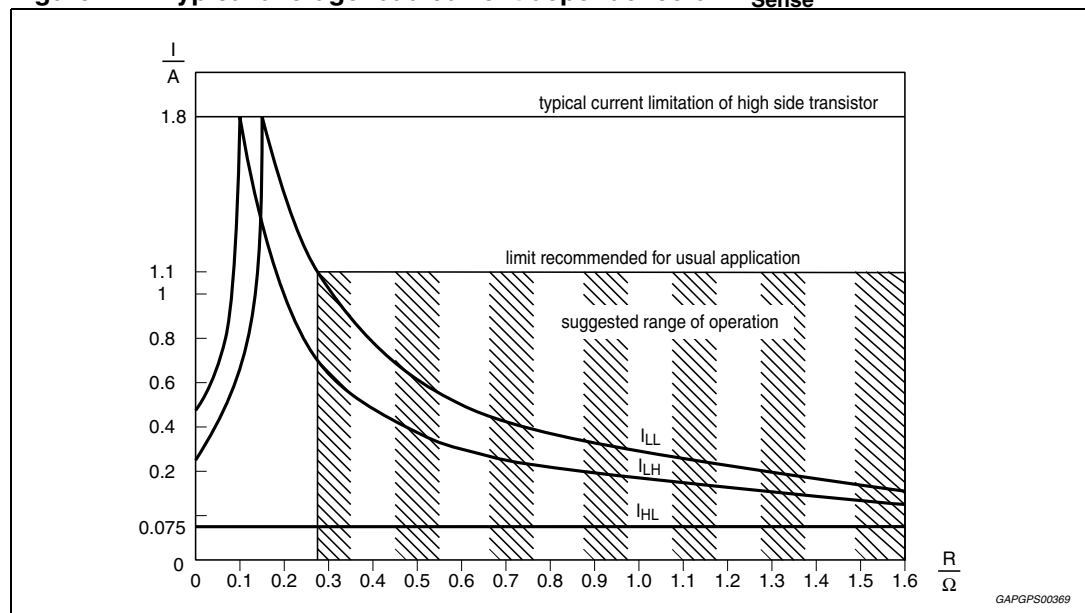
Figure 4. Typical average load current dependence on R_{\text{Sense}}
