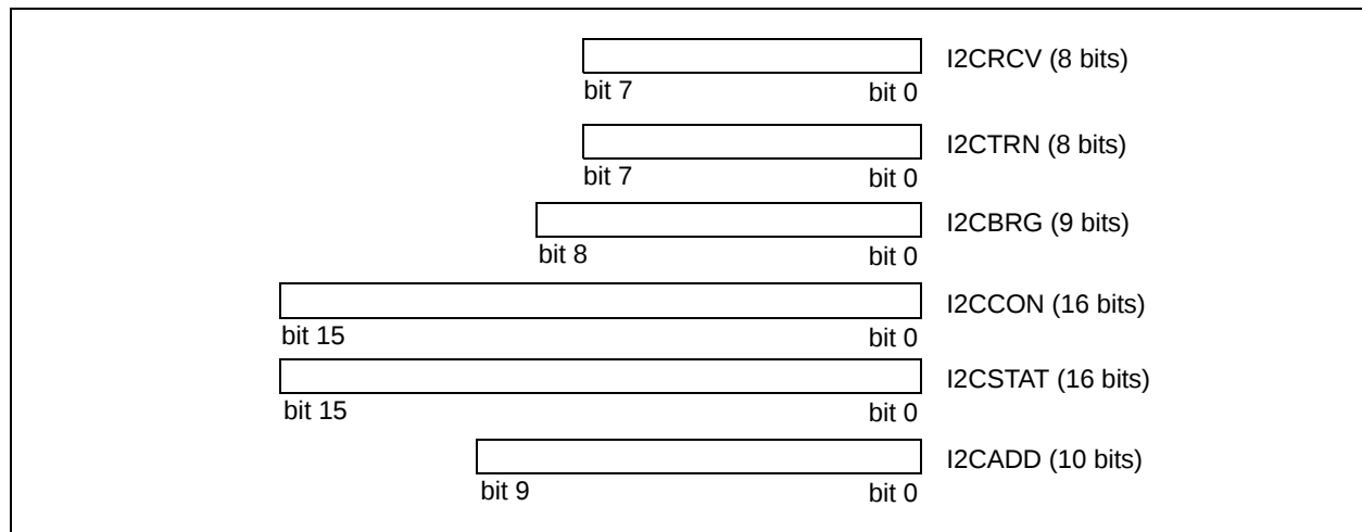
FIGURE 17-1: PROGRAMMER’S MODEL
