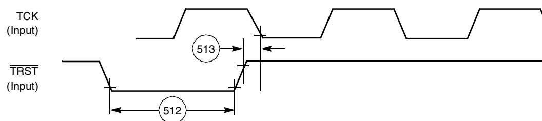
Figure 2-47. \overline{\text{TRST}} Timing Diagram
