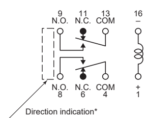
Schematic (Bottom view)
