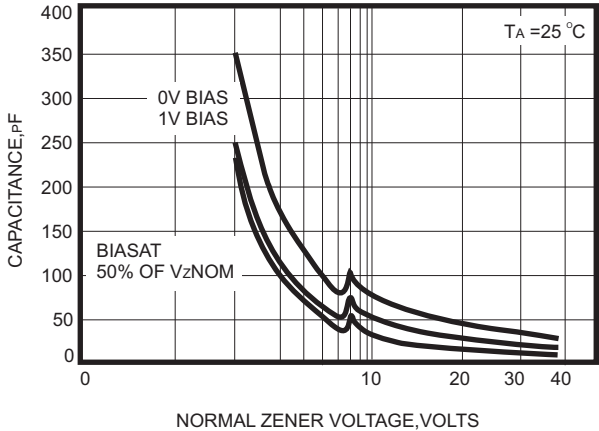
Fig.6 TYPICAL CAPACITANCE
