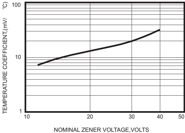
Fig.2 TEMPERATURE COEFFICENTS
