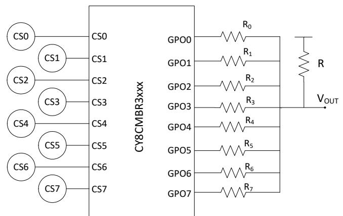
Figure 12. Voltage Output Using GPO and Resistor Network
