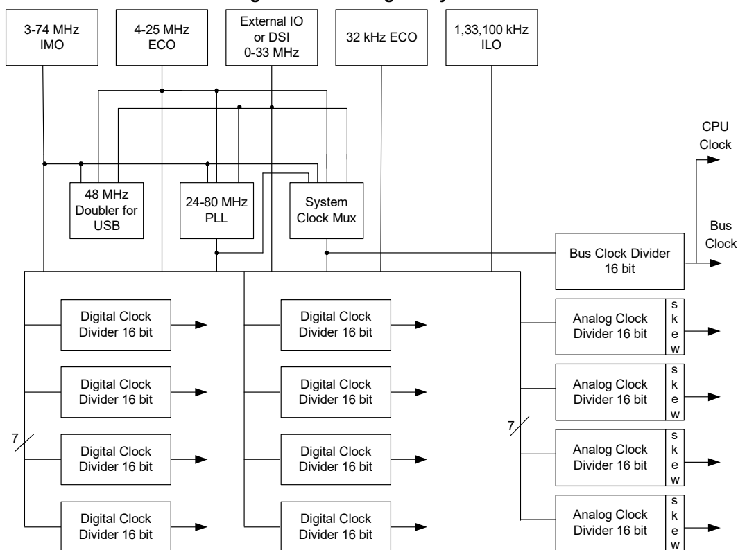
Figure 6-1. Clocking Subsystem
