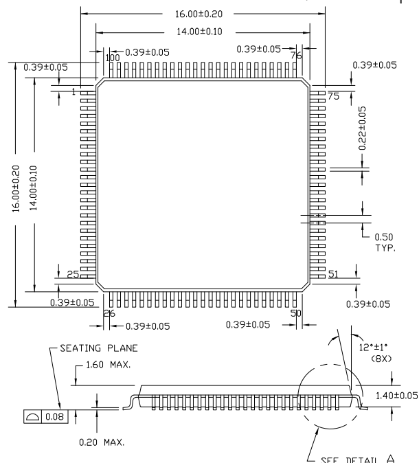
Figure 21. 100-pin TQFP (14 × 14 × 1.4 mm) A100SA Package Outline, 51-85048
