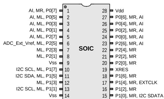
Figure 3. Pin Diagram
