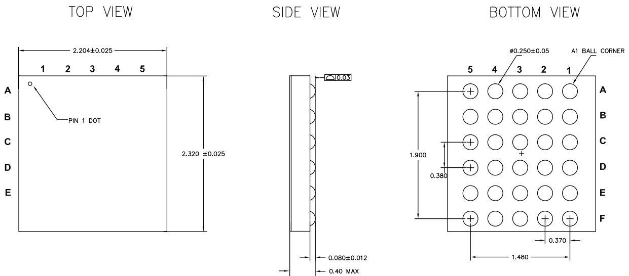
Figure 21. 30-pin WLCSP
