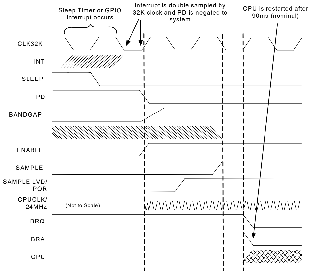
Figure 15-2. Wakeup Timing
