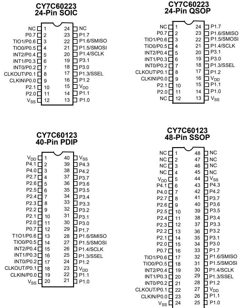
Figure 7-1. Package Configurations Top View
