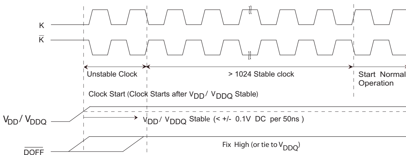
Figure 3. Power-up Waveforms
