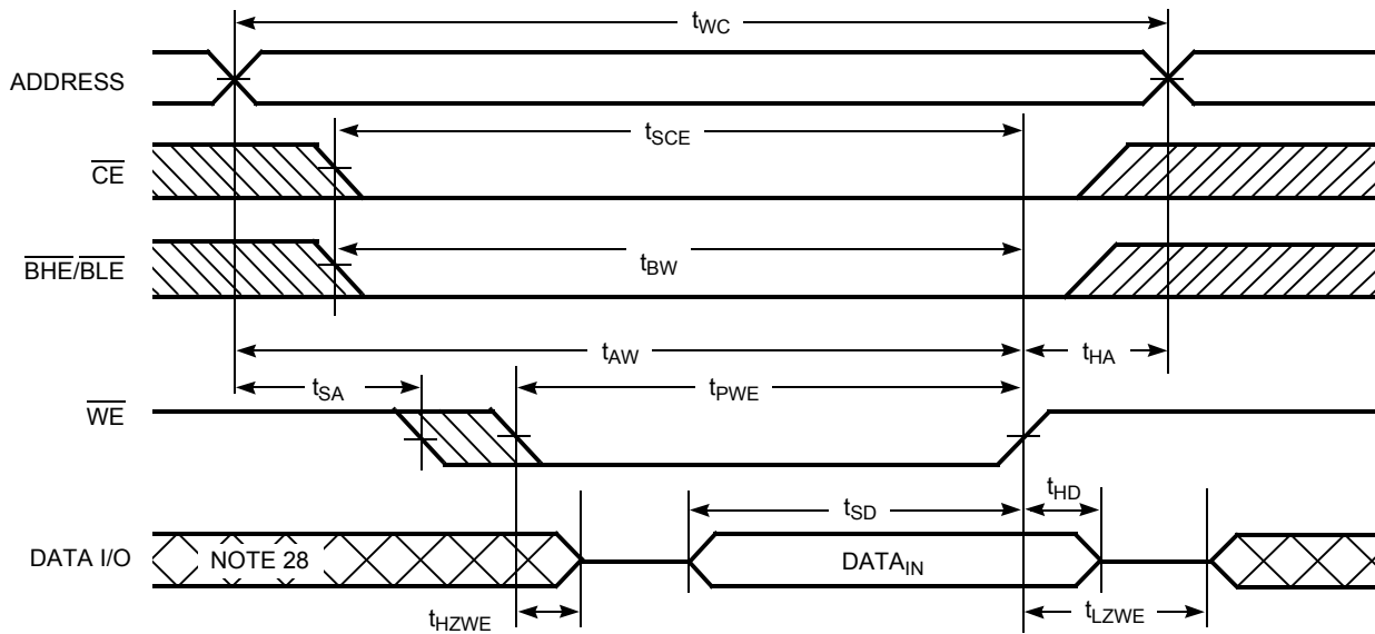
Figure 10. Write Cycle No. 4 ( \overline{BHE/BLK} controlled, \overline{OE} LOW) [26]
