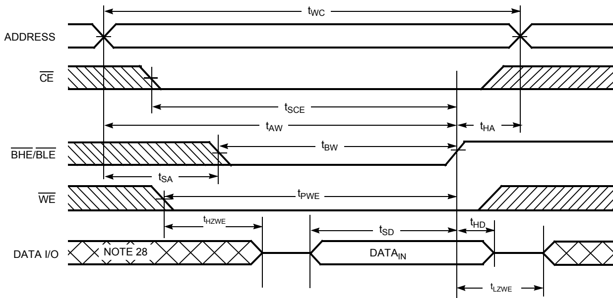
Figure 10. Write Cycle No. 4 ( \overline{BHE/BLK} controlled, \overline{OE} LOW) [26]
