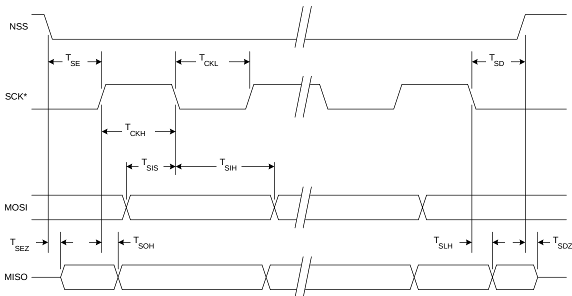
Figure 16.11. SPI Slave Timing (CKPHA = 1)
