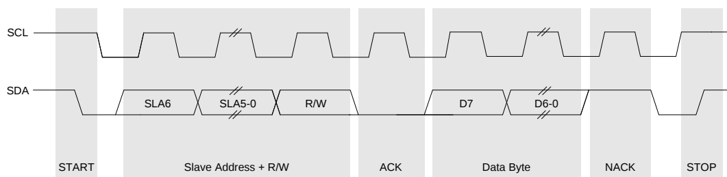
Figure 14.3. SMBus Transaction
