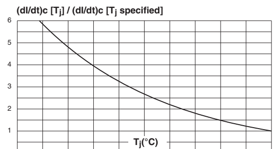
Figure 10. Relative variation of critical rate of decrease of main current versus T_j
