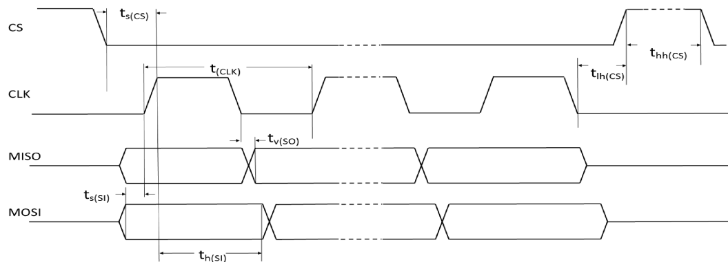
Figure 14. SPI timings
