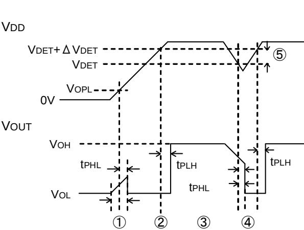
Fig.14 Timing Waveform
