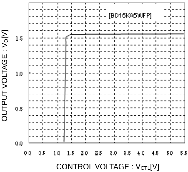
Fig.15 CTL Voltage vs. Output Voltage
