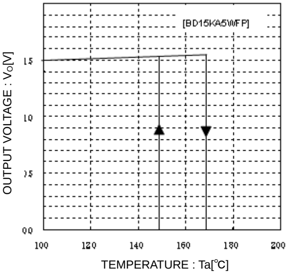
Fig.17 Thermal Shutdown Circuit Characteristics ( I_o=5\text{mA} )
