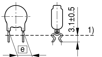
1) Seating plane to IEC 60717 VAR0413-V
