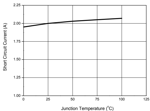
Figure 10. Short Circuit Current vs. Junction Temperature
