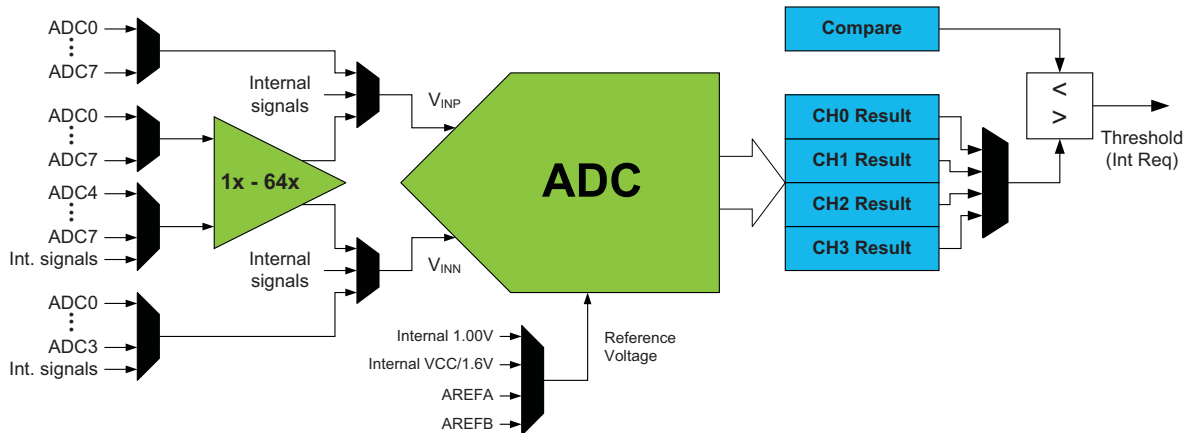
Figure 26-1. ADC overview
