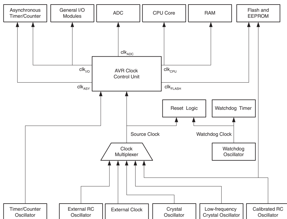
Figure 8-1. Clock Distribution
