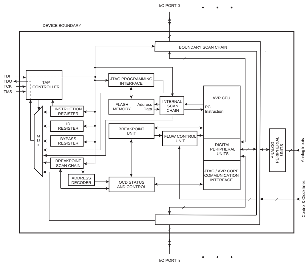
Figure 23-1. Block Diagram
