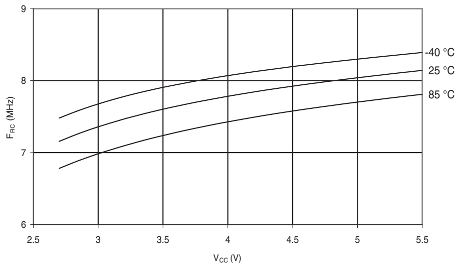
Figure 28-38. Calibrated 8MHz RC Oscillator Frequency vs. V_{CC}
