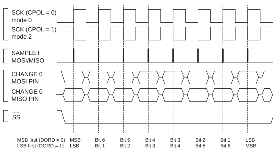
Figure 18-2. SPI Transfer Format with CPHA = 0
