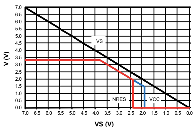
Figure 4-8. VCC and NRES versus VS (Ramp-down) for 3.3V (SBC and Voltage Regulator)
