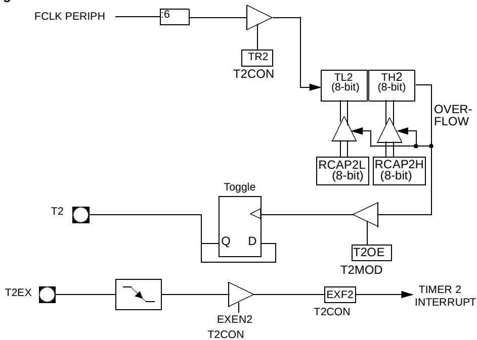
Figure 10. Clock-Out Mode C/\overline{T2} = 0
