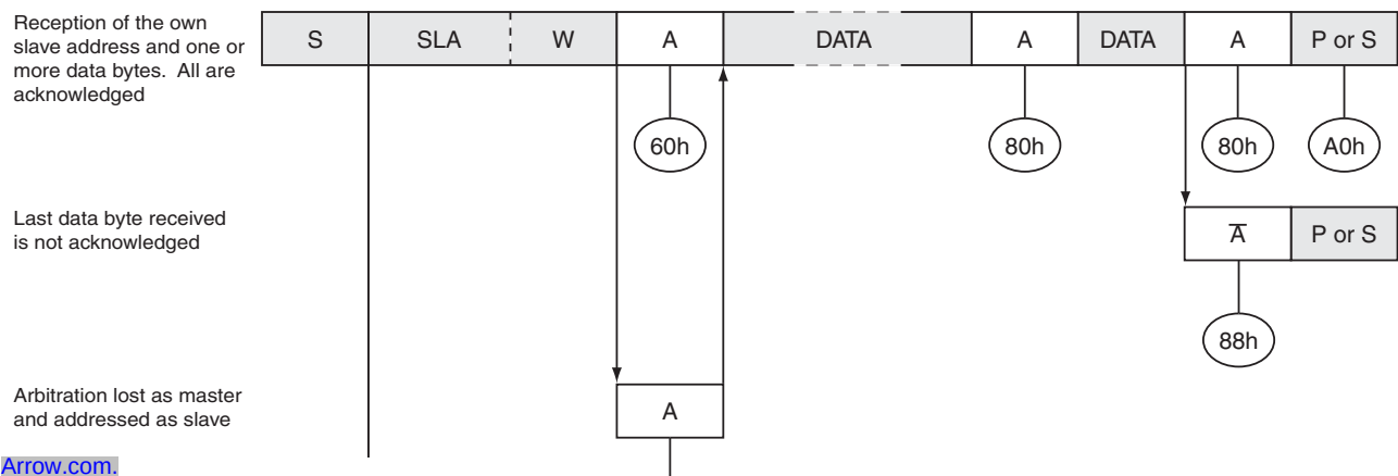
Figure 18-13. Format and States in Slave Receiver Mode
