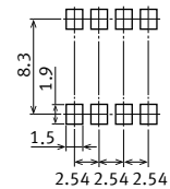
Recommended mounting pad (TOP VIEW)
