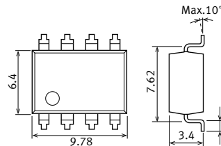
Surface mount terminal type External dimensions
