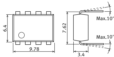
Through hole terminal type External dimensions
