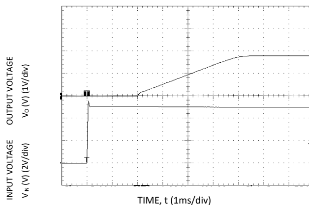
Figure 18. Typical Start-up Using Input Voltage ( V_{IN} = 5V , I_o = I_{o,max} ).
