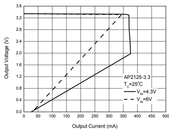
Figure 11. Current Limit
