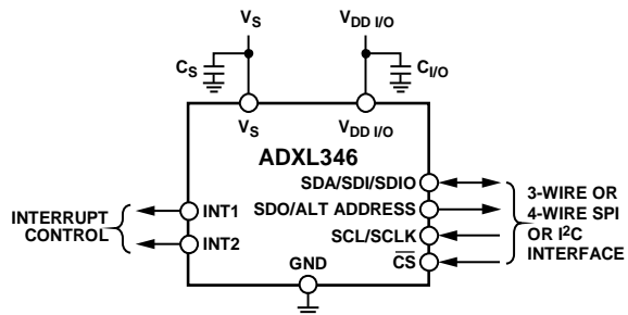
Figure 44. Applications Diagram
