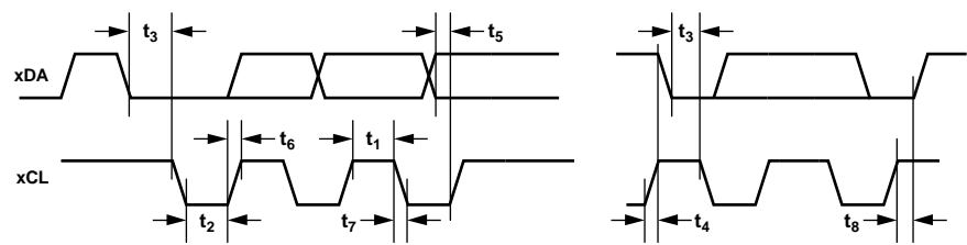
Figure 2. I²C Timing
