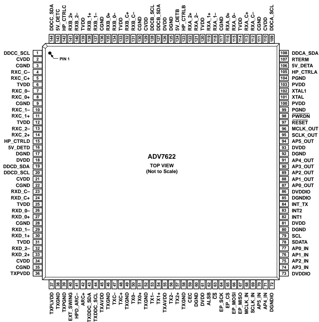
Figure 5. Pin Configuration
