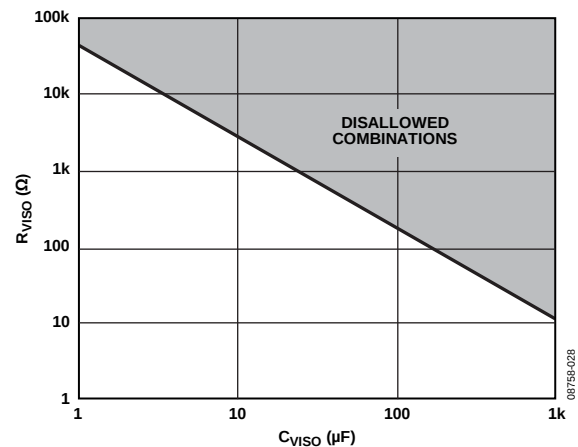
Figure 29. Maximum Capacitive Load for Proper Restart
