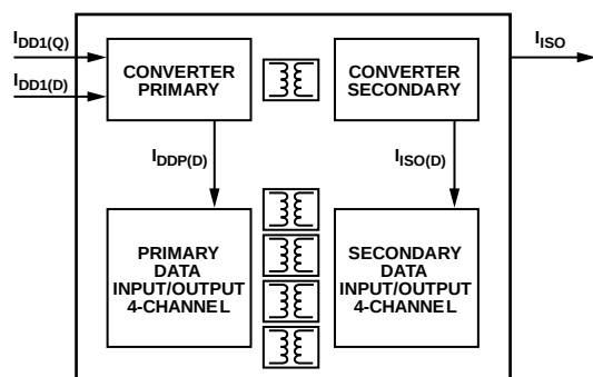
Figure 25. Power Consumption Within the ADuM5401W/ADuM5402W/ADuM5403W
