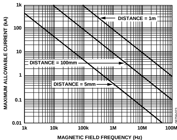
Figure 24. Maximum Allowable Current for Various Current-to-ADuM5401W/ADuM5402W/ADuM5403W Spacings
