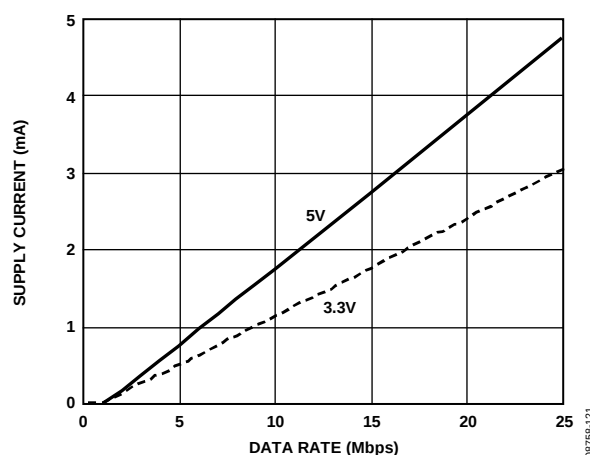
Figure 19. Typical I_{ISO(D)} Dynamic Supply Current per Input
