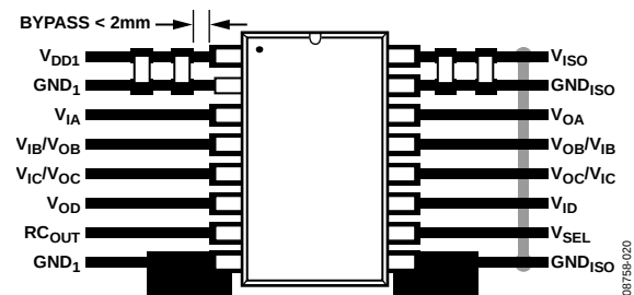
Figure 21. Recommended Printed Circuit Board Layout
