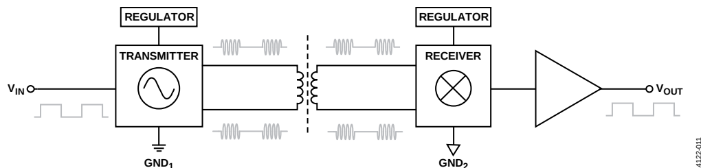
Figure 13. Operational Block Diagram of a Single Channel with a Low Fail-Safe Output State
