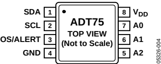
Figure 4. Pin Configuration
