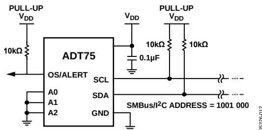
Figure 13. Typical SMBus/I 2 C Interface Connection
