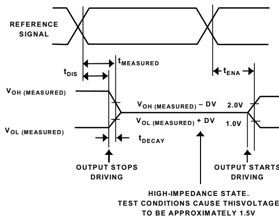
Figure 32. Output Enable/Disable
