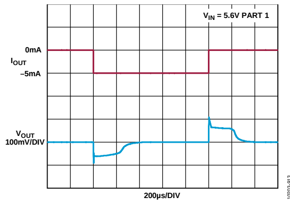
Figure 81. ADR4540 A, B, C Grade Load Transient Response (Sourcing)
