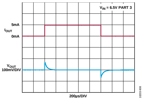
Figure 99. ADR4550 A, B, C Grade Load Transient Response (Sinking)
