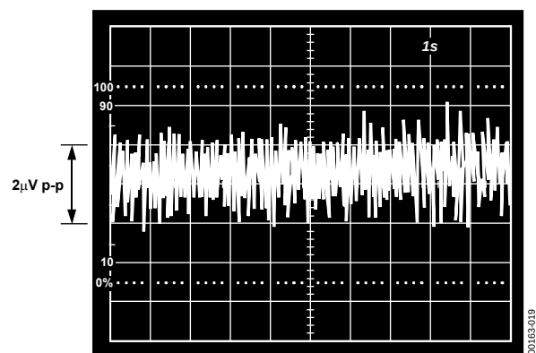
Figure 22. ADR291 0.1 Hz to 10 Hz Noise
