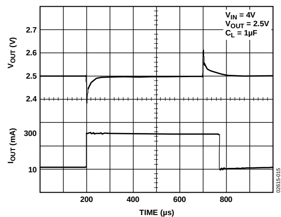
Figure 15. Load Transient Response, C_L = 1 \mu F
