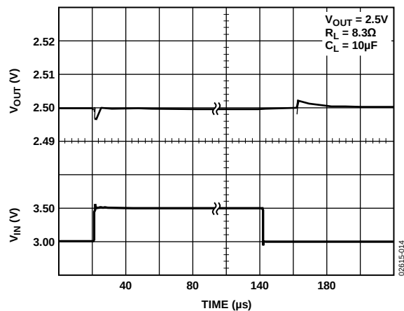
Figure 14. Line Transient Response, C_L = 10 \mu F
