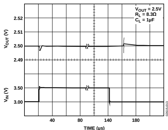
Figure 13. Line Transient Response, C_L = 1 \mu F
