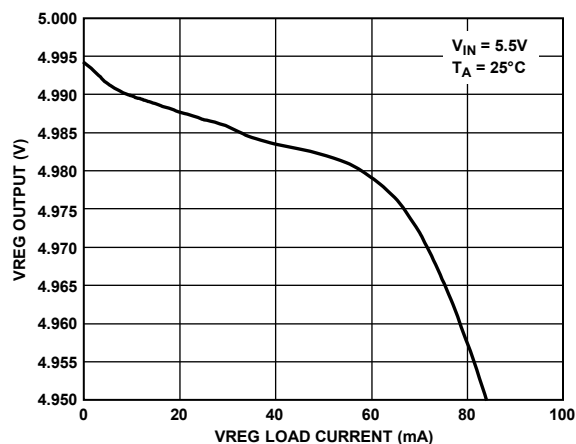
Figure 11. VREG vs. Load Current
