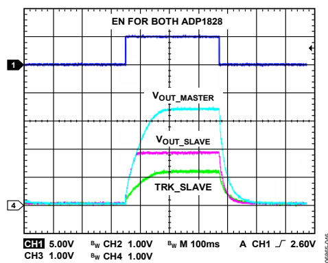
Figure 45. Coincident Tracking of Figure 43
