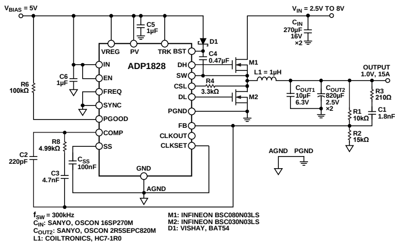
Figure 56. Application Circuit for V_{IN} = 2.5\text{ V} TO 8 V
