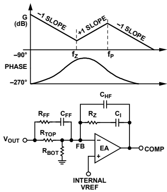
Figure 40. Type III Compensation
