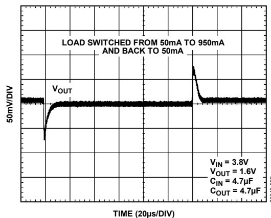
Figure 19. Load Transient Response, C_{IN} = 4.7 \mu F , C_{OUT} = 4.7 \mu F
