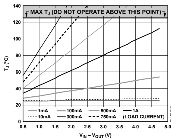
Figure 40. 100 mm 2 of PCB Copper, T_A = 25^{\circ}\text{C} , LFCSP
