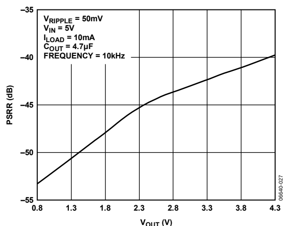
Figure 26. ADP1708 Power Supply Rejection Ratio vs. Output Voltage
