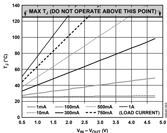
Figure 36. 500 mm 2 of PCB Copper, T_A = 25^{\circ}\text{C} , SOIC
