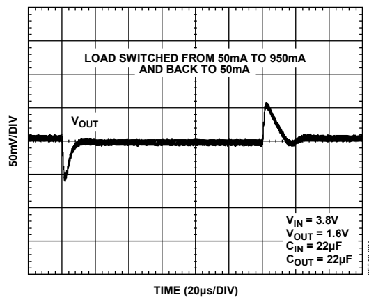
Figure 20. Load Transient Response, C_{IN} = 22 \mu F , C_{OUT} = 22 \mu F
