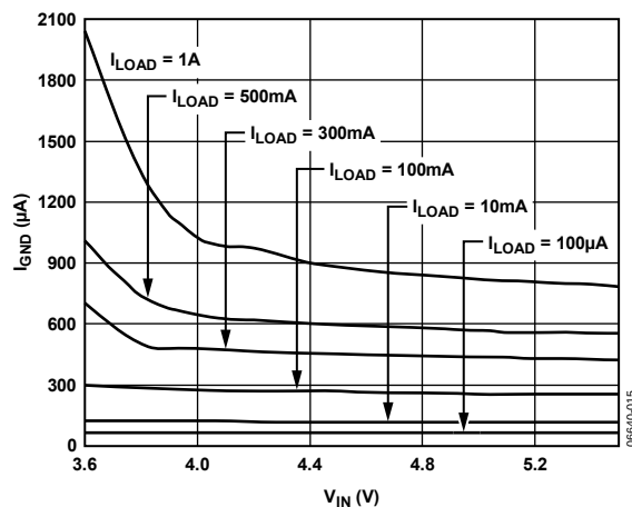
Figure 15. Ground Current vs. Input Voltage
