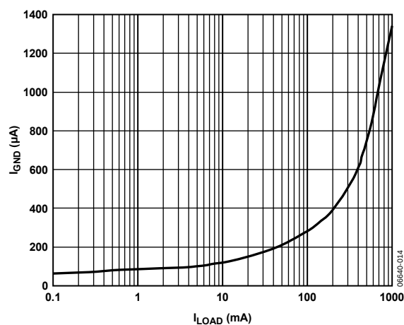
Figure 14. Ground Current vs. Load Current
