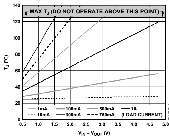
Figure 41. 0 mm 2 of PCB Copper, T_A = 25^{\circ}\text{C} , LFCSP
