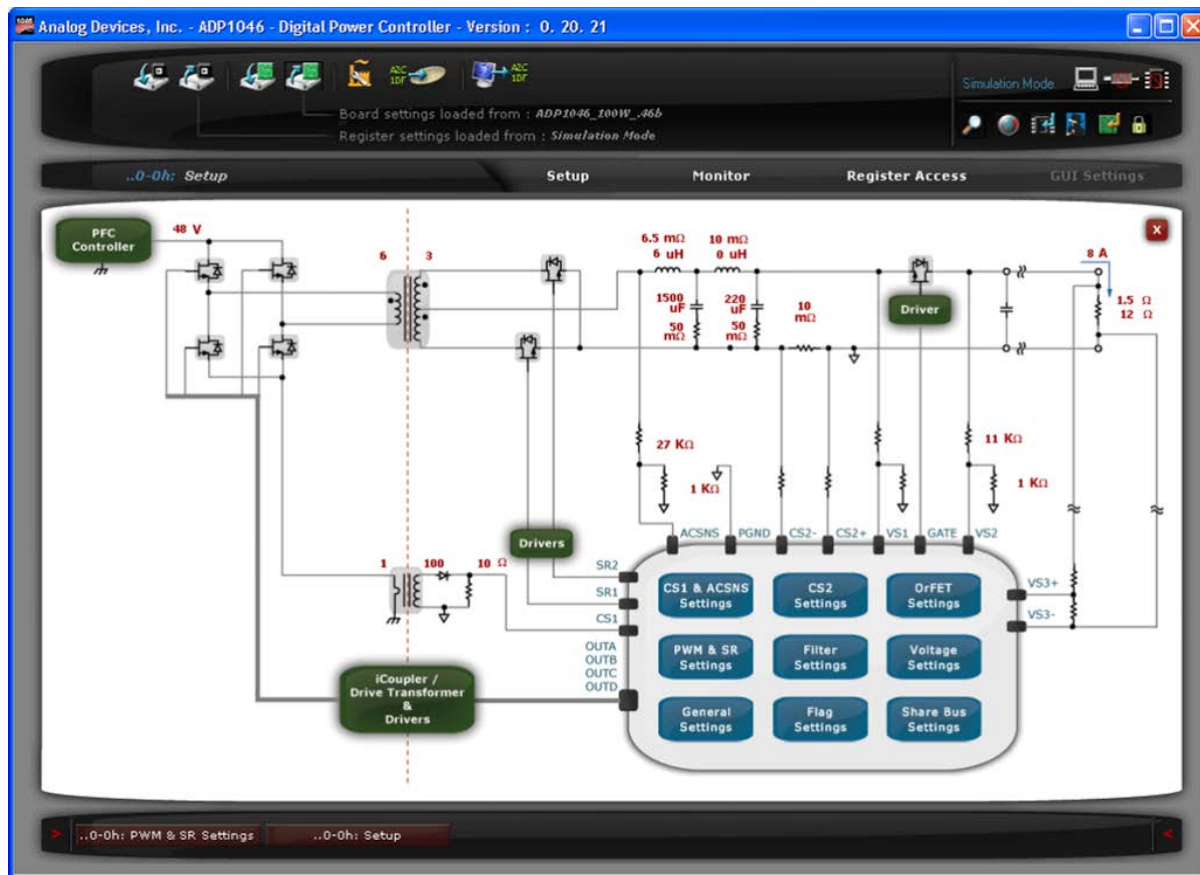
Figure 55. ADP1046 GUI
