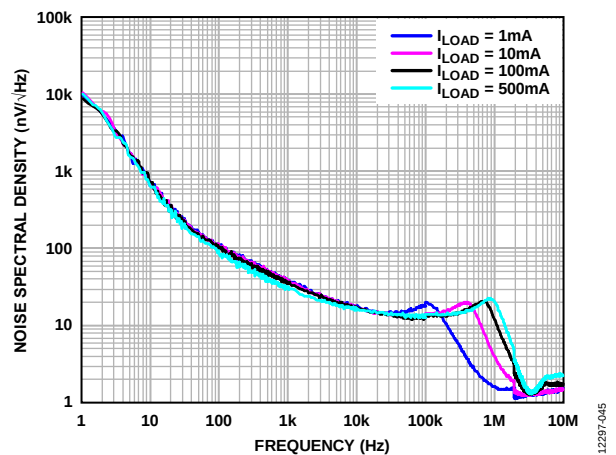
Figure 45. Output Noise Spectral Density, V_{OUT} = 3\text{ V}
