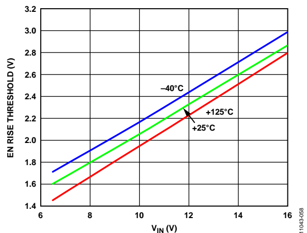
Figure 58. Typical EN Rise Threshold vs. Input Voltage ( V_{\text{IN}} ) for Various Temperatures
