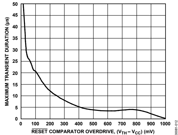
Figure 7. Maximum Transient Duration vs. RESET Comparator Overdrive
