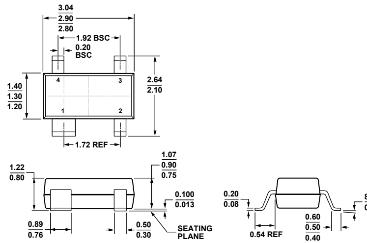
Figure 12. 4-Lead Small Outline Transistor Package [SOT-143] (RA-4)
