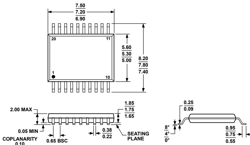
Figure 25. 20-Lead Shrink Small Outline Package [SSOP]
