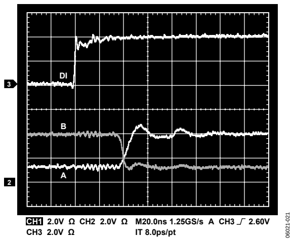
Figure 12. Driver/Receiver Propagation Delay, Low to High ( R_{LDIFF} = 54\text{ }\Omega , C_{L1} = C_{L2} = 100\text{ pF} )
