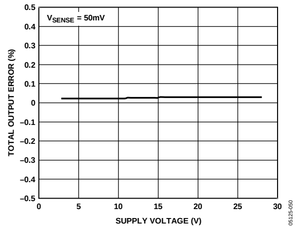
Figure 33 CSOUT Total Output Error vs. Supply Voltage
