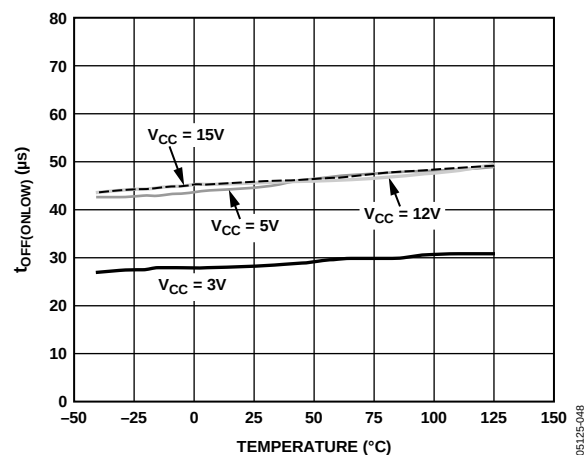
Figure 25. t_{OFF(ONLOW)} vs. Temperature
