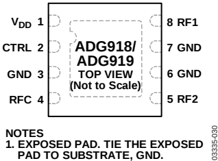
Figure 5. ADG918/ADG919 Pin Configuration (LFCSP)
