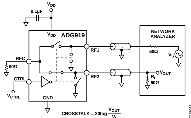
Figure 23. Crosstalk
