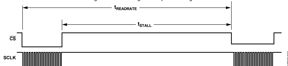
Figure 3. Stall Time and Data Rate Timing Diagram
