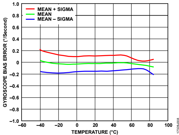
Figure 11. Gyroscopic Bias Error vs. Temperature, ADIS16505-2, All Axes
