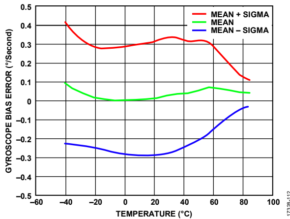
Figure 12. Gyroscopic Bias Error vs. Temperature, ADIS16505-3, All Axes
