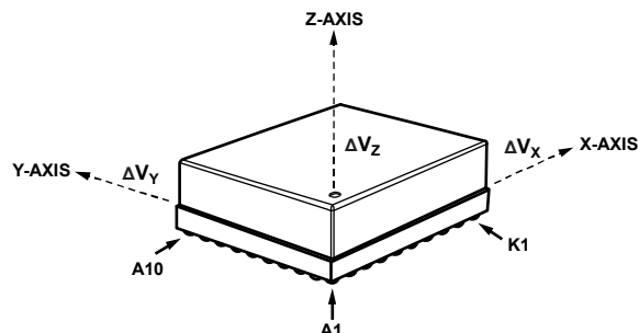
Figure 54. Delta Velocity Axis and Polarity Assignments
