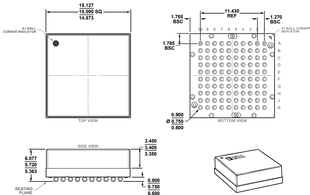
Figure 66. 100-Ball Ball Grid Array Module [BGA] (ML-100-1)
