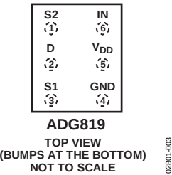
Figure 3. 6-Ball WLCSP Pin Configuration
